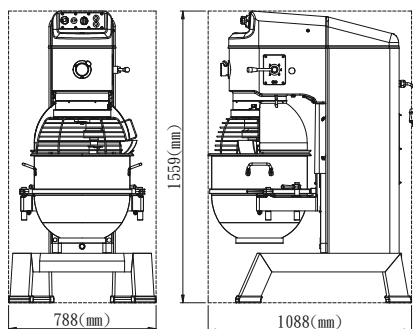
(SP-A80HI/SP-B80HI) DIMENSION
