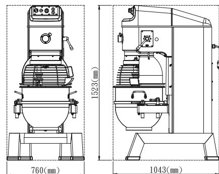
(SP-62P/SP-B62P) DIMENSION
